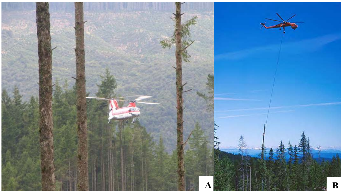
Figure 11: A - Helicopter thinning operation along the margins of a lake in New Zealand. Photo courtesy of Timberland Limited. B – Sikorski (now Erikson) S-64E skycrane lifting a prepared stem from a riparian reserve. Note the tops of prepared stems are also visible. Photo courtesy of FPInnovations FERIC division.
