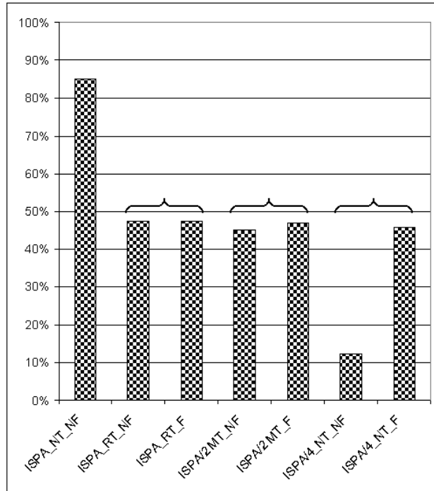
FIG. 7—Conformance of seven regimes to a 3.5-km/sec lower specification limit on acoustic velocity.
