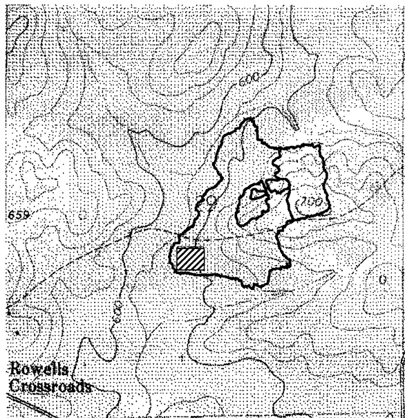
FIG. 1—Relative locations of harvested loblolly pine plantation (dark outline) and grid point sampling systems (hatched square) in the Piedmont region of Alabama, United States (Map Source: 7.5 Minute U.S. Geological Survey (USGS) Quadrangle Map, Section 29 of Waverly, Alabama quadrangle).
