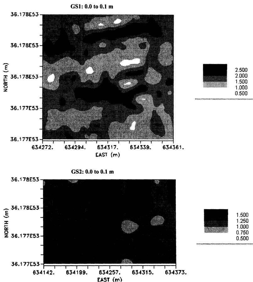
FIG. 4—Contour maps of punctual kriged cone index values (MPa) of soil surface layers at two grid spacings: 3 \times 6 m (GS1) and 28 \times 28 m (GS2) in a harvested loblolly pine plantation, Alabama.
