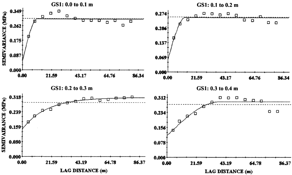
FIG. 2—Isotropic semivariograms of cone index values (MPa) by soil depth evaluated on a 3 × 6 m grid spacing (GS1) in a harvested loblolly pine plantation, Alabama.
