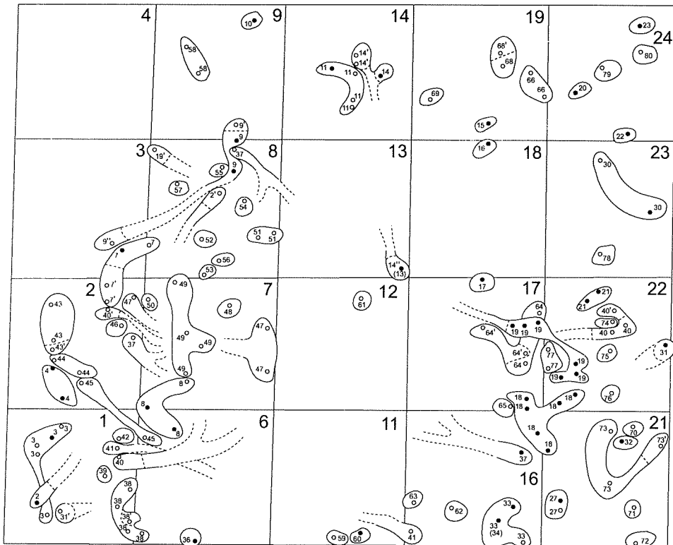
FIG. 6—Distribution of Armillaria isolates taken from trees, dead (solid circles) or living (hollow circles), between 1990 and 1993 (stand age 5–7 years; first isolation series). Large numerals are plot numbers. Small figures denote separate compatibility groups or colonies (genets; those shared with Fig. 7 are the same; numbers with ' signs indicate possible additional genets suggested during cultural pairing). Groups, as known, are delineated by encircling solid or (where more distant) solid and broken lines.
