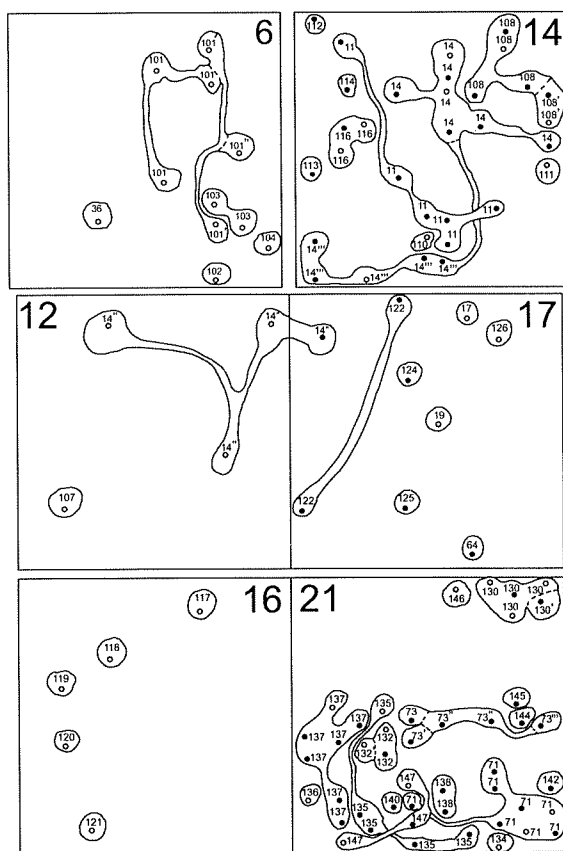
FIG. 7—Distribution of Armillaria isolates taken from infected trees or colonised stumps in six selected plots in February and March 1998 (stand age 12.5 years, nearly 6 years after thinning to 250 stems / ha; second isolation series). Large numerals are plot numbers (Treatment 3 plots, no stumps, are to the left and Treatment 2 plots, with stumps, to the right). Small figures denote separate compatibility groups or colonies (genets; numerals <100 shared with Fig. 6; numbers with ' signs indicate possible additional genets suggested during cultural pairing). Solid circles represent thinning stumps (Plots 14, 17, 21, only) and hollow circles living trees
