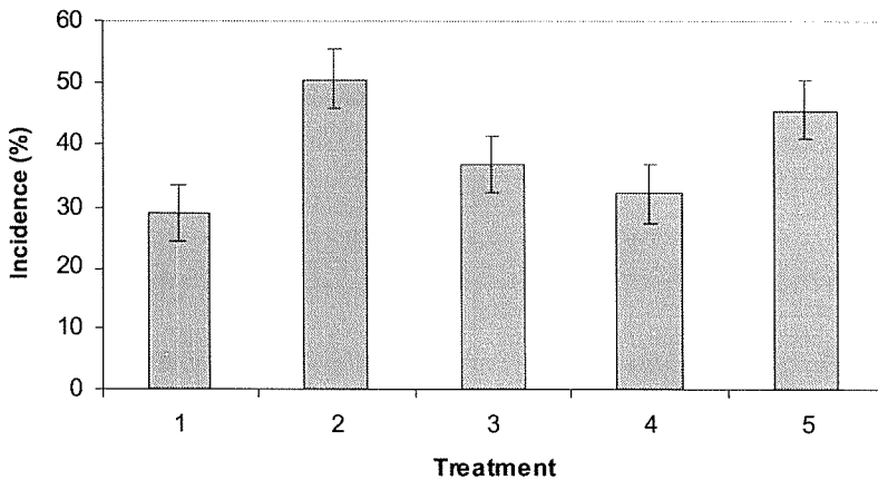
FIG. 4—Mean percentage incidence of trees infected by Armillaria species at age 12.5 years, adjusted for pre-thinning incidence at age 6 years (error bars indicate standard errors). Treatment numbers: 1 = unthinned, unpruned; 2 = thinned to 250 stems/ha, pruned; 3 = thinned to 250 stems/ha, pruned, no stumps; 4 = unthinned, pruned; 5 = thinned to 500 stems/ha, pruned. Treatments 2 ( p , 0.007) and 5 ( p , 0.029) differ significantly from Treatment 1 (control); Treatments 3 and 4 do not.
