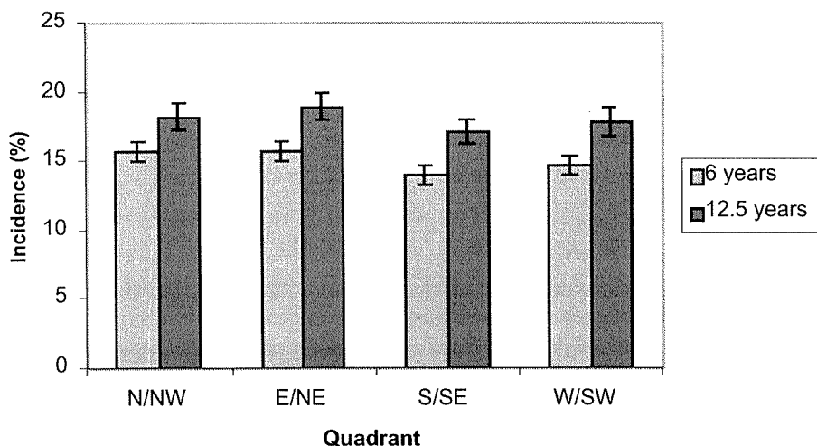
FIG. 5—Direction of infection around trees at stand age 6 years (1991–92) and, after thinning, at 12.5 years (1997–98) (percentage girdling midpoint incidence for each quadrant; error bars indicate standard errors).
